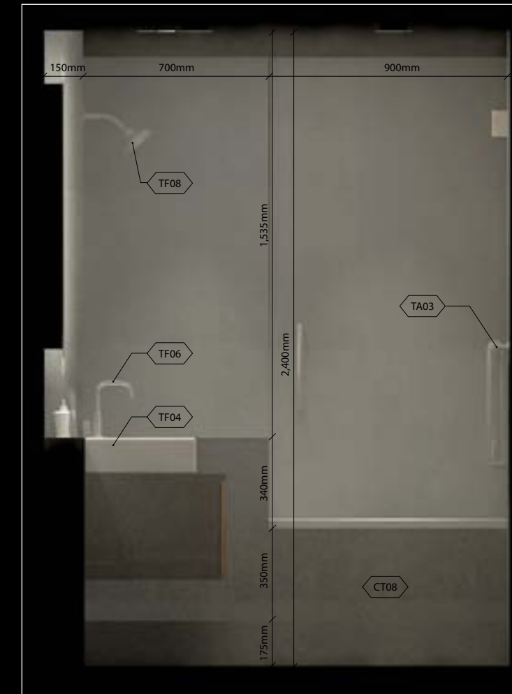
Interior Elevation 3 Scale 1:20
