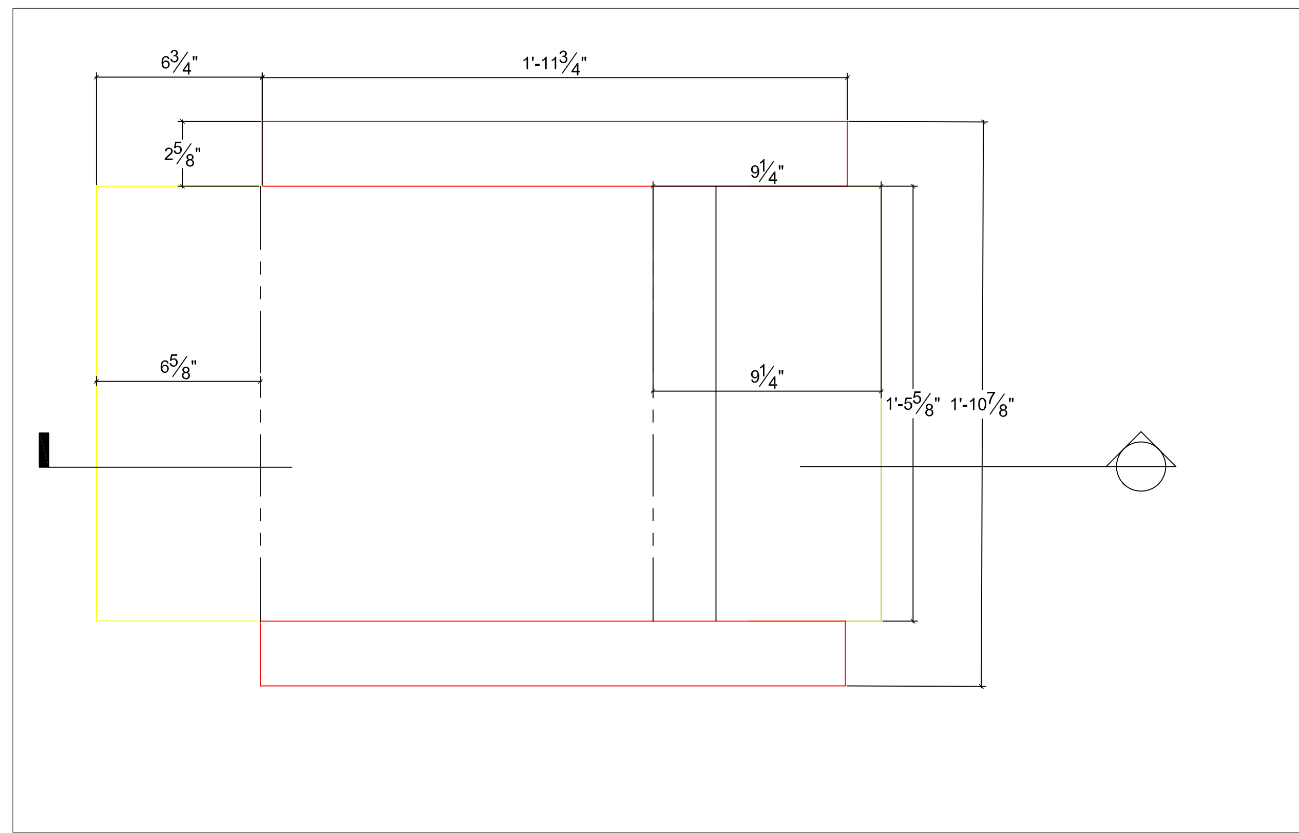
2 PLAN A-100.00 DRAWING SCALE (I.E. 1/4"=1'-0")
