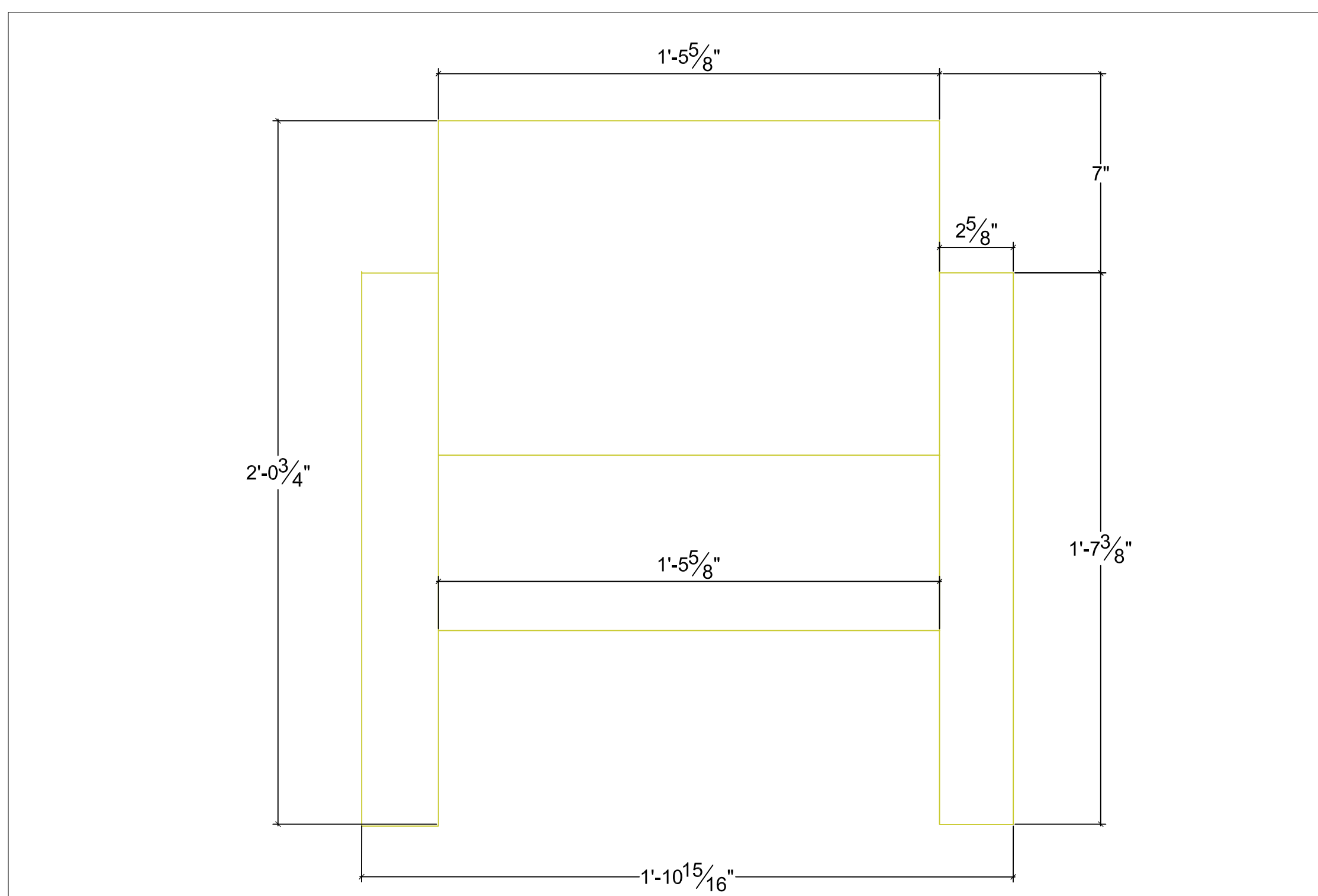
3 FRONT ELEVATION A-100.00 DRAWING SCALE (I.E. 1"=1'-0")
