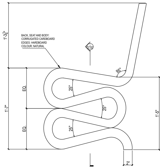
3 A-100.00 ELEVATION B DRAWING SCALE 3"=1'-0"
