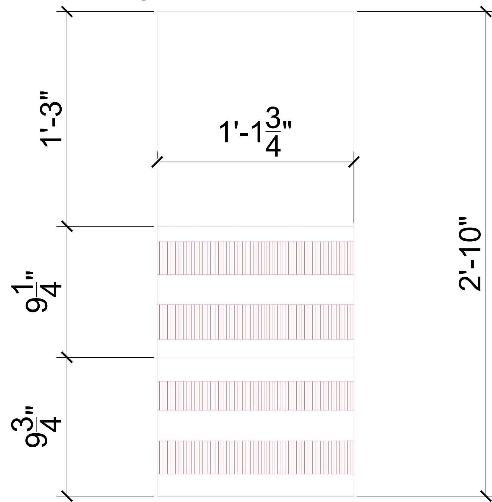
1 CHAIR SECTION ELEVATION DRAWING SCALE (I.E. 1/4"=1'-0")
