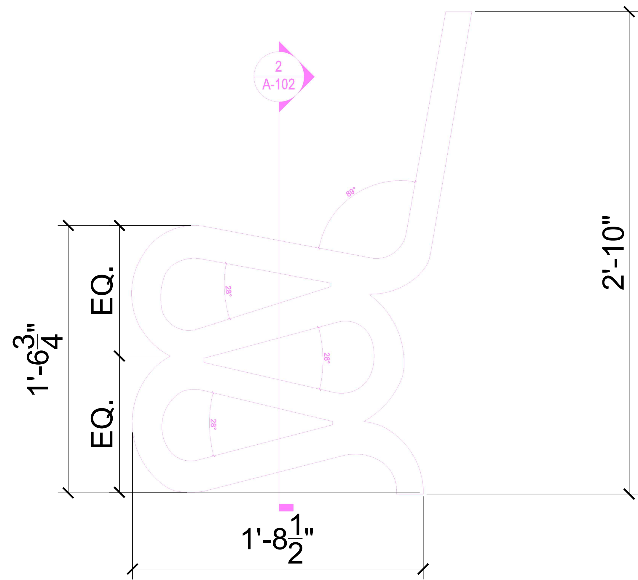
1 CHAIR SECTION ELEVATION DRAWING SCALE (I.E. 1/4"=1'-0")
