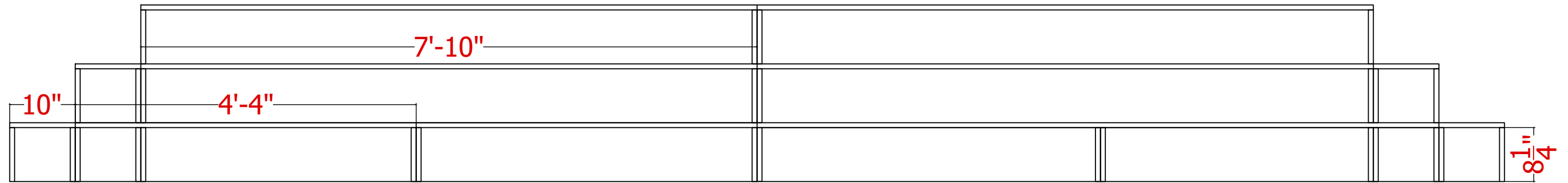
2 Front Staircase - Front View \frac{3}{4} "-1'-0"
