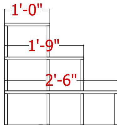
3 Front Staircase - Section View \frac{3}{4} "-1'-0"
