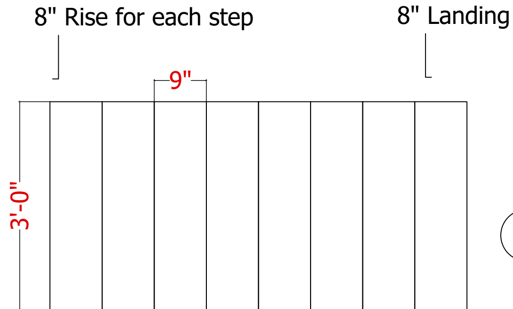
1 Back Staircase - Top View
