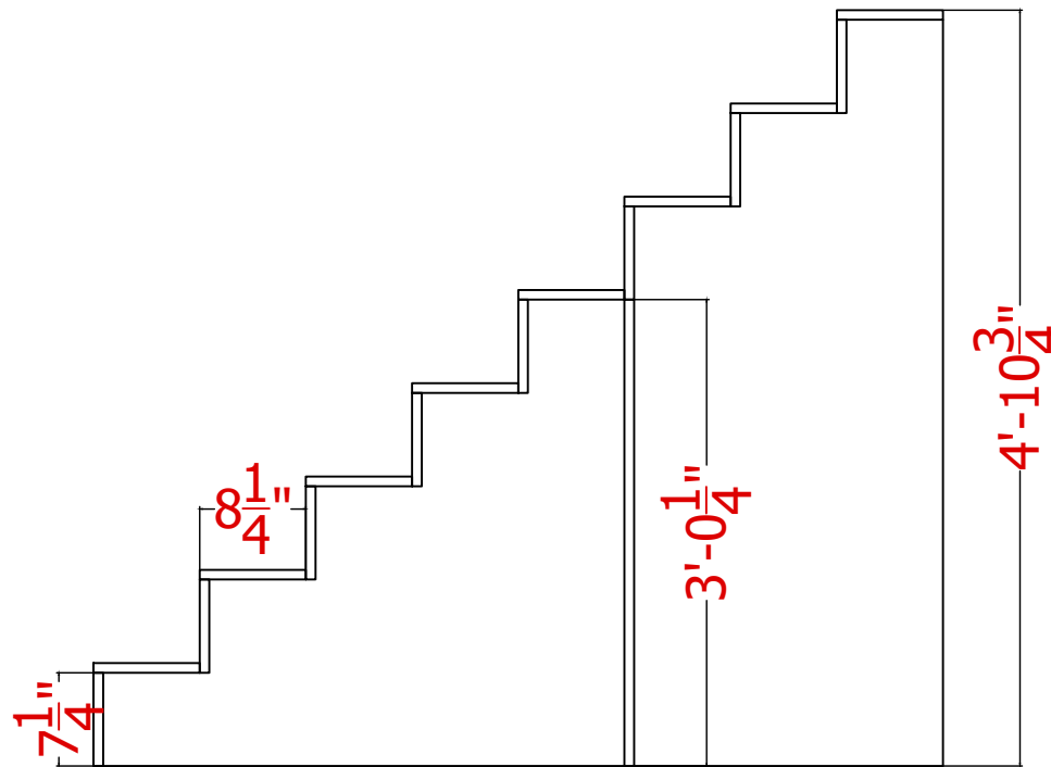
2 Back Staircase - Section View
