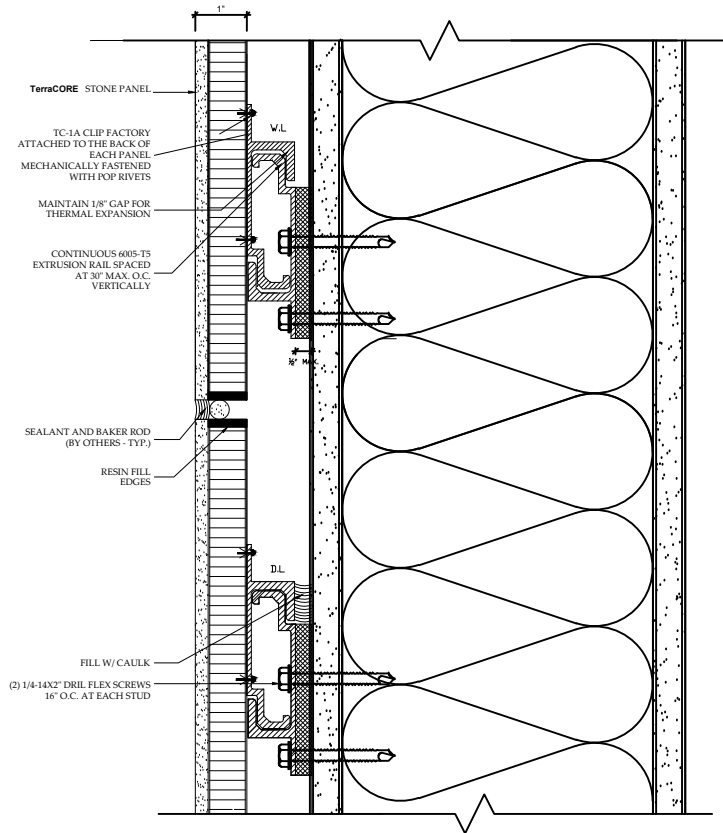
TYPICAL TC STONE PANEL JOINT
