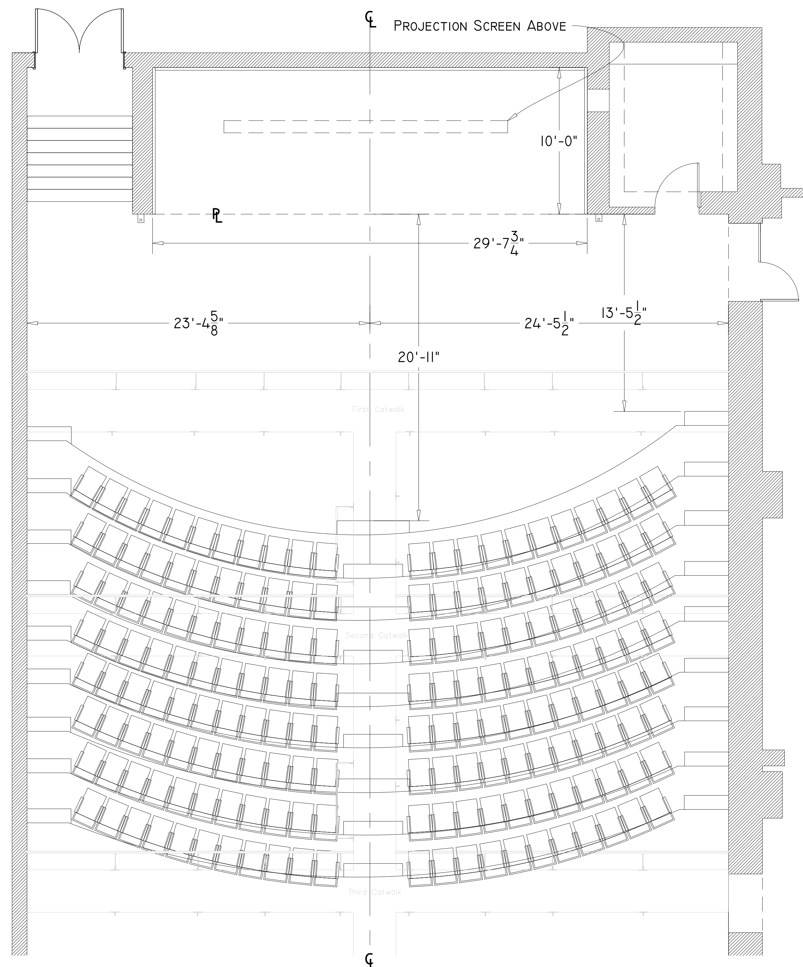
1 GROUND PLAN
