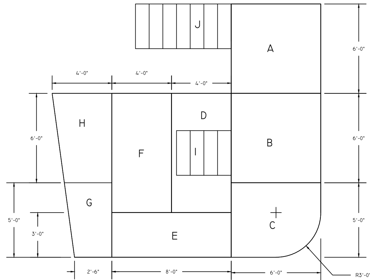
PLATFORM INSTALLATION UNITS
