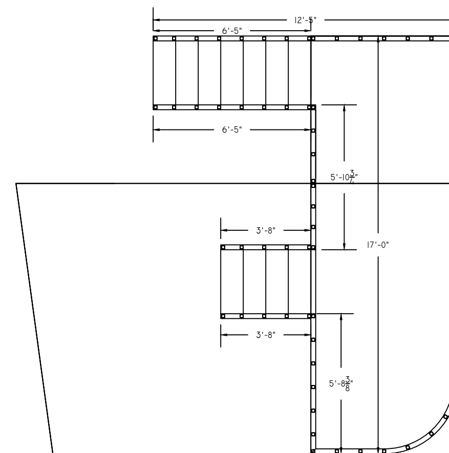
HANDRAILS & BALUSTERS LOCATION
