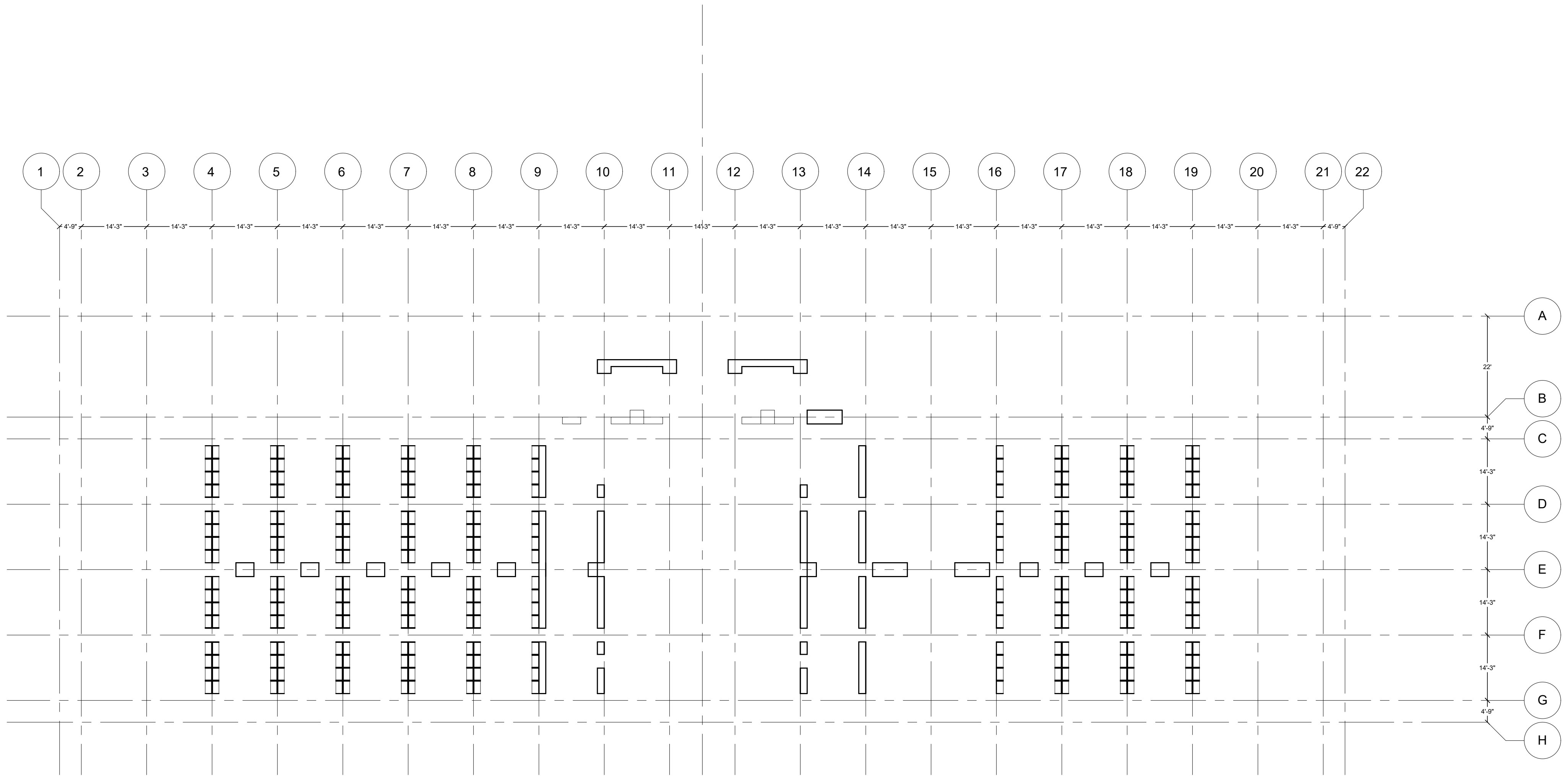
BIBLIOTHEQUE S. GENEVIEVE PLAN UNDERLAY: GRID + MILLWORK +PARTITION ARCH 1230_MONTGOMERY_2017_10_21_SINGH_RYAN
