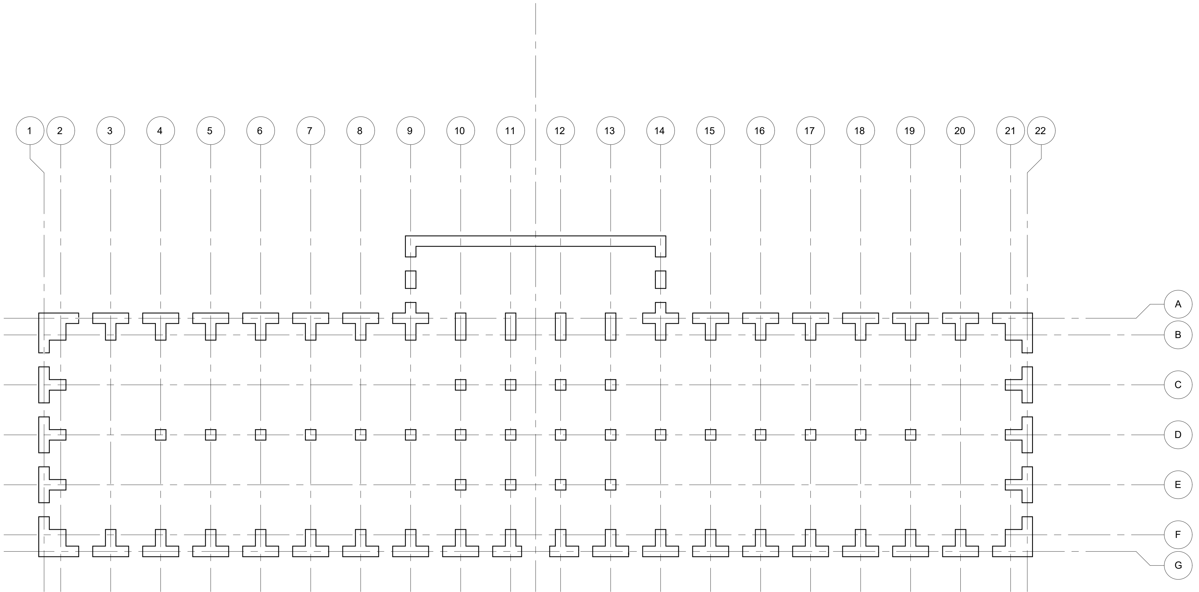
BIBLIOTHEQUE S. GENEVIEVE PLAN OVERLAY: GRID + STRUCTURE ARCH 1230_MONTGOMERY_2017_10_21_SINGH_RYAN
