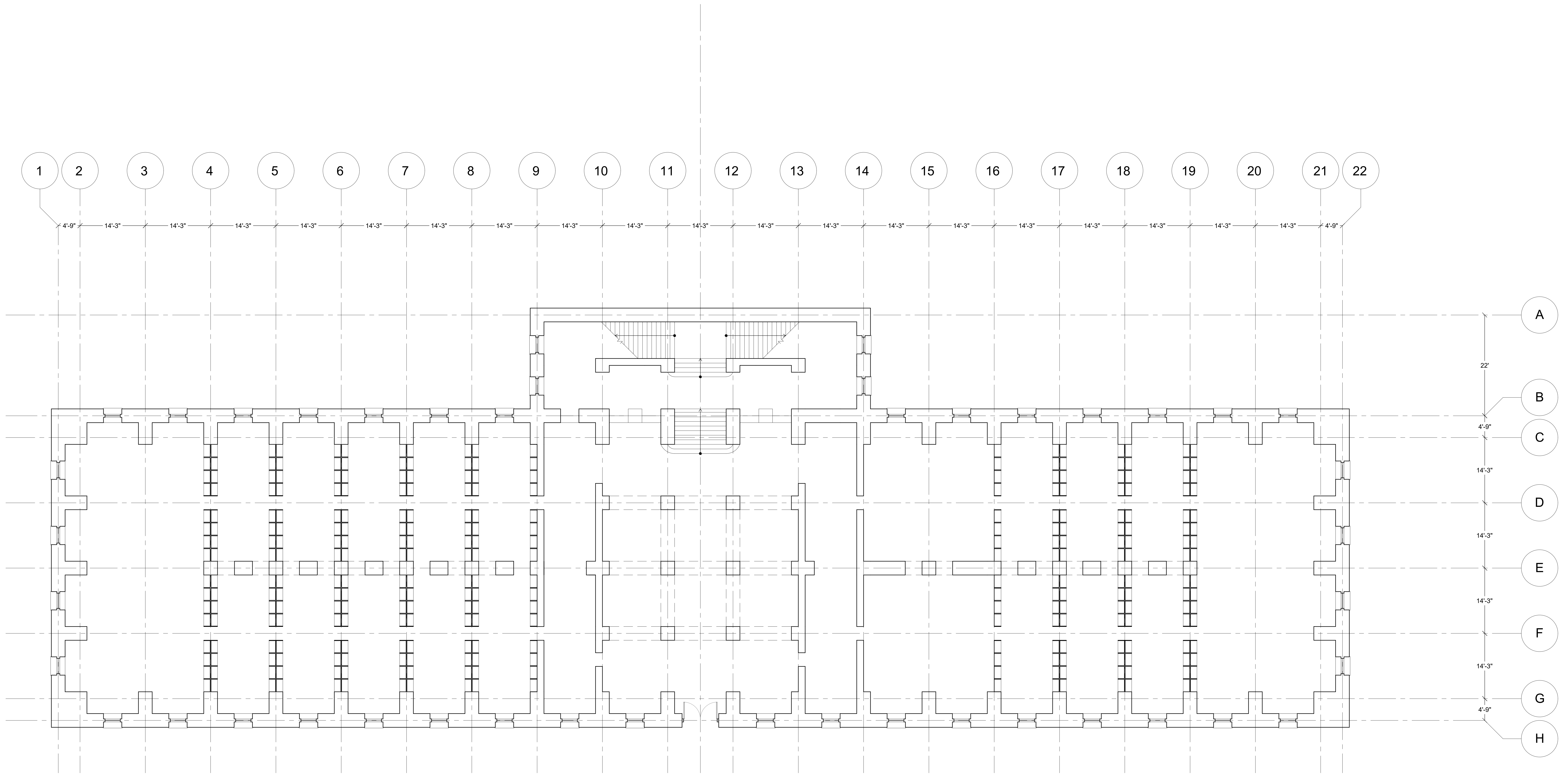
BIBLIOTHEQUE S. GENEVIEVE GROUND FLOOR PLAN
