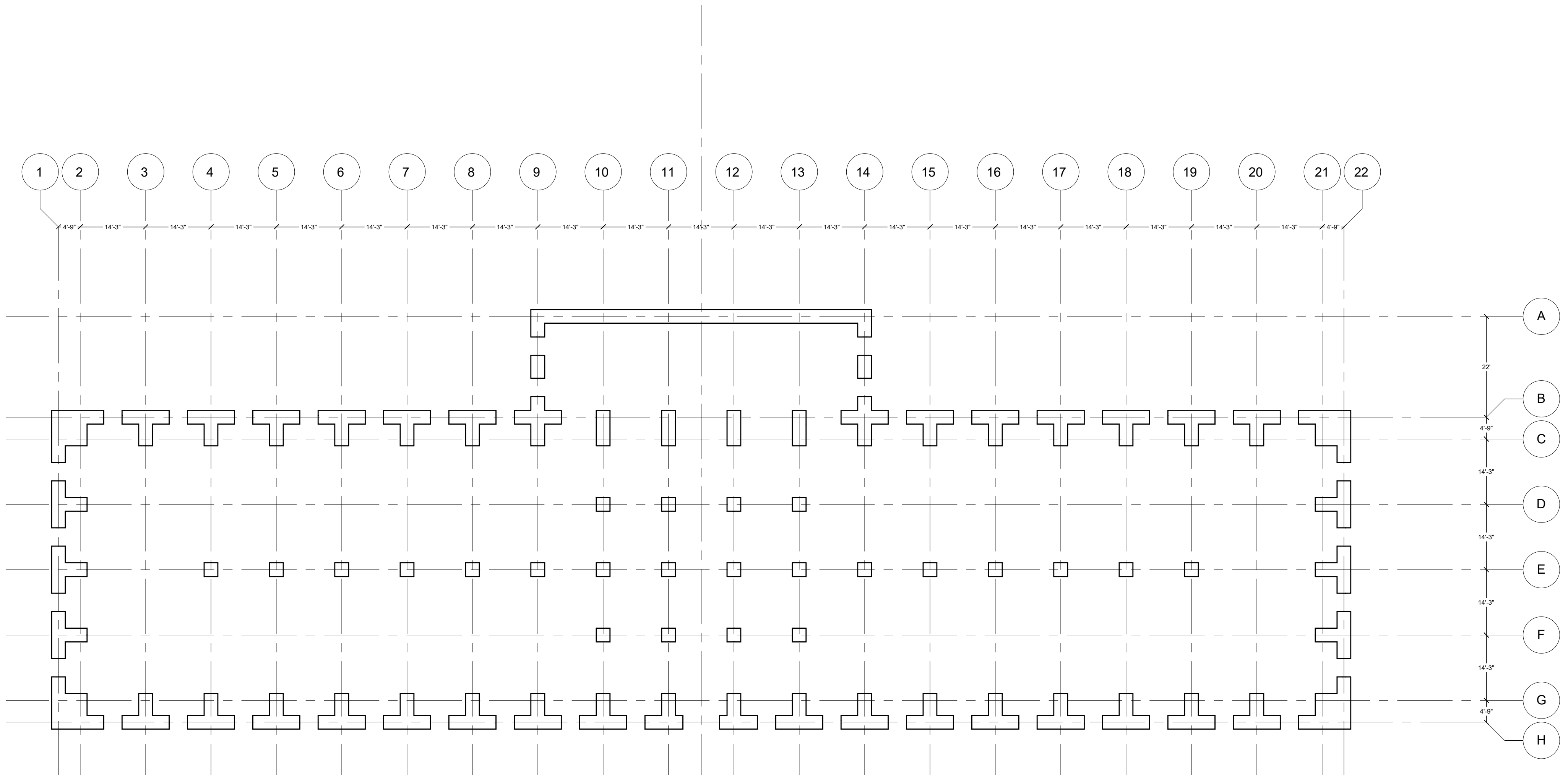
BIBLIOTHEQUE S. GENEVIEVE PLAN UNDERLAY: GRID + STRUCTURE ARCH 1230_MONTGOMERY_2017_10_21_SINGH_RYAN
