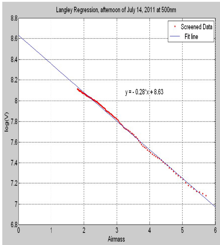
Fig.1. A Langley plot showing the negative slope which is the Total Optical Depth and the approximate extraterrestrial solar constant (y-int.) .
