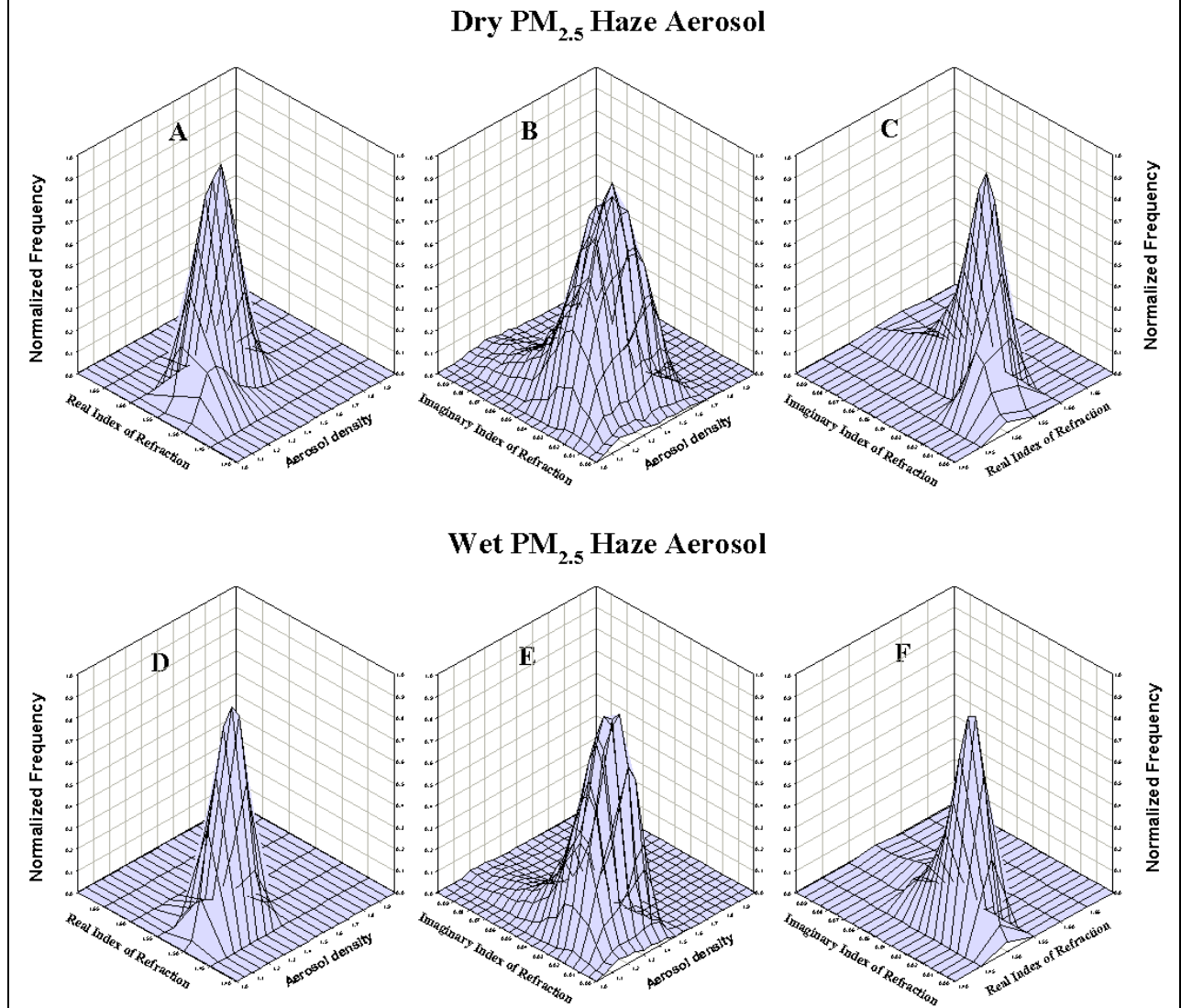
Figure 3. Normalized joint frequency distributions of aerosol physical parameters ( \rho, n, k ) for IMPROVE data set dry and wet PM 2.5 haze aerosol. Wet aerosol calculated with semi-empirical water uptake model at RH=40\% .
