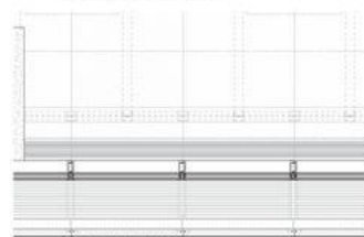
CURTAIN WALL PLAN
