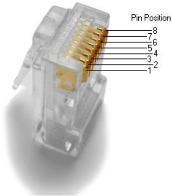
RJ45 Crimpable Connectors for CAT-5e
