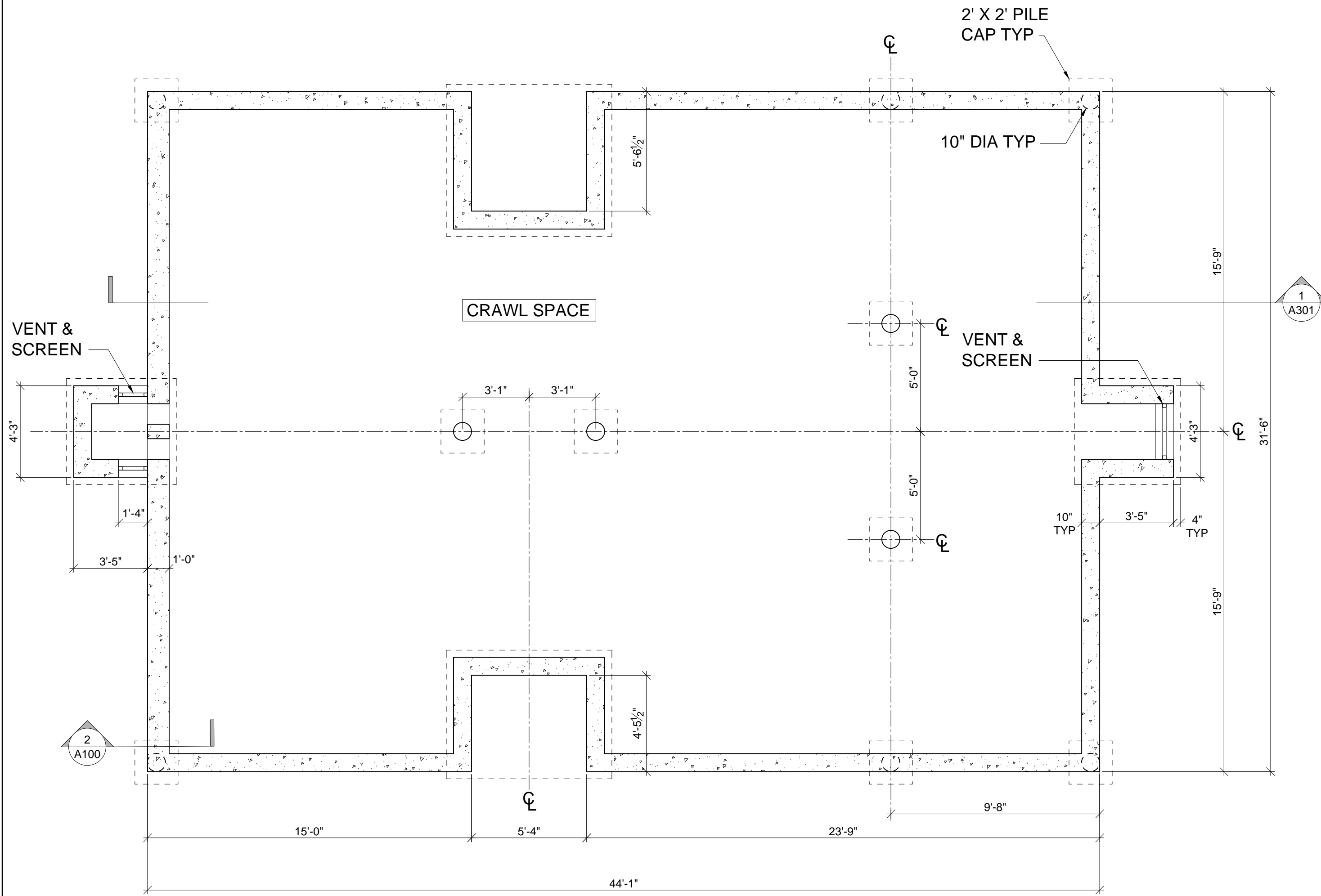
1 CELLAR PLAN 1/4" = 1'-0"
