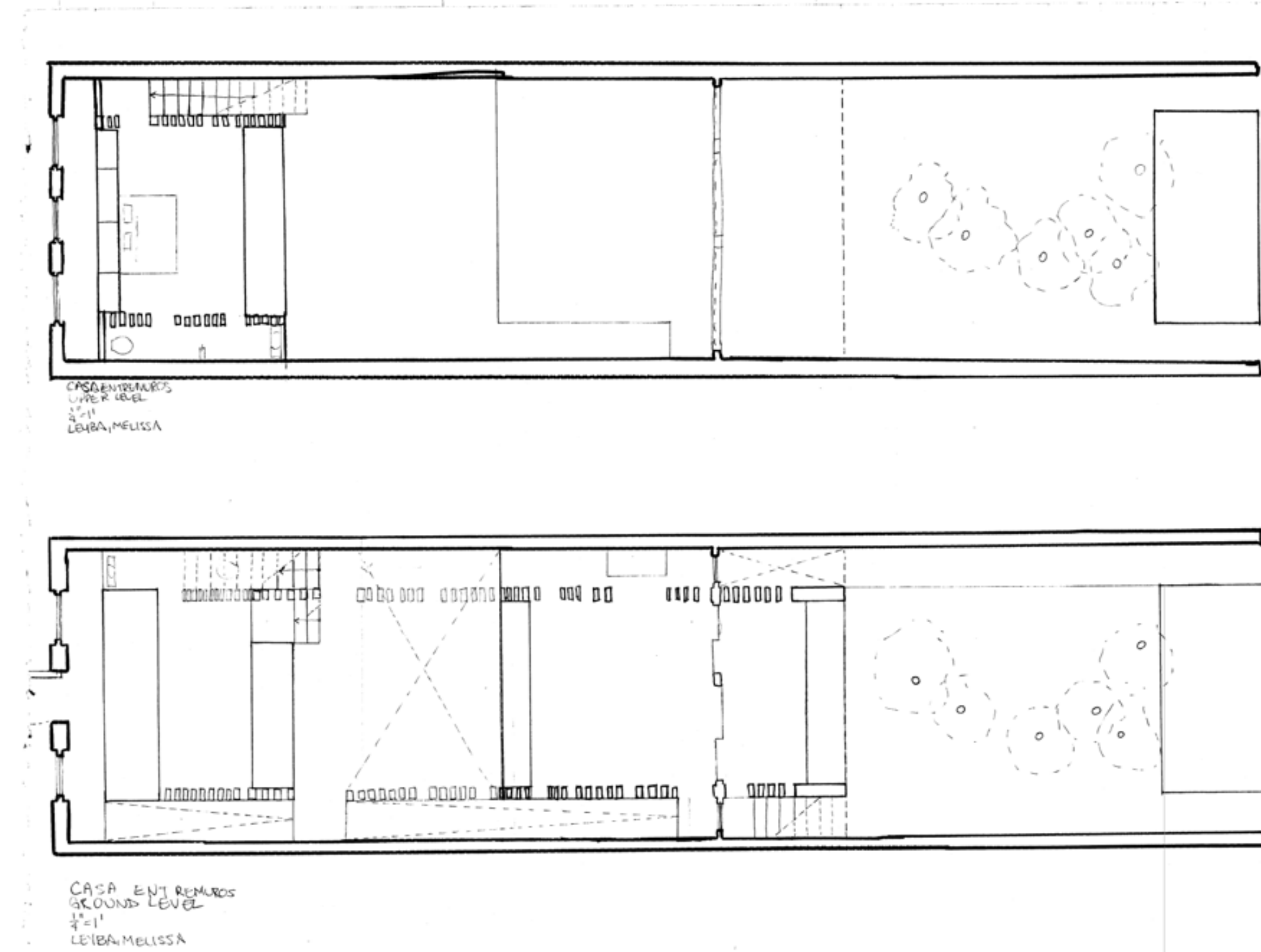
FLOOR PLANS
