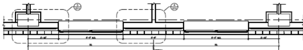
2 PARTIAL PLAN @ WINDOW (TYPICAL @ BRICK) SCALE 1/4"=1'-0"
