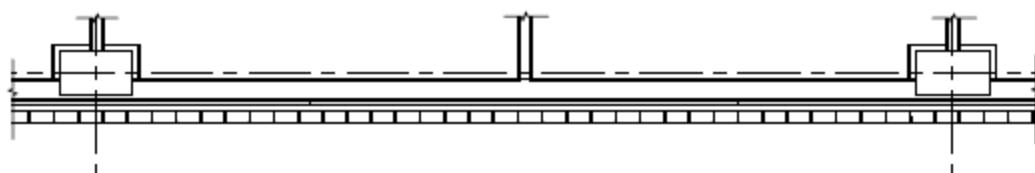
3 PARTIAL PLAN @ BELOW WINDOW (TYPICAL @ BRICK) SCALE 1/4"=1'-0"
