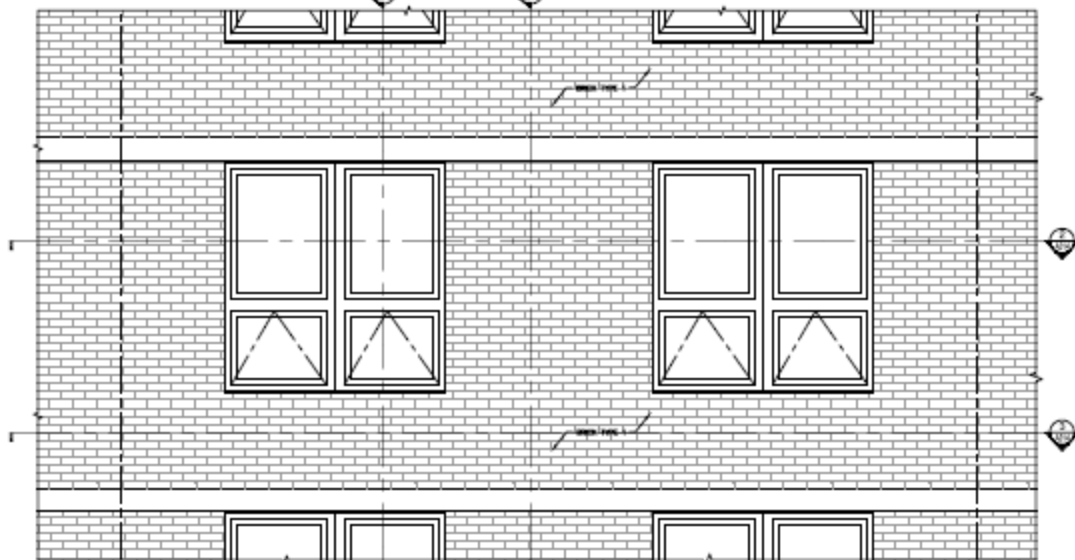
1 PARTIAL ELEVATION (TYPICAL @ BRICK) SCALE 1/4"=1'-0"
