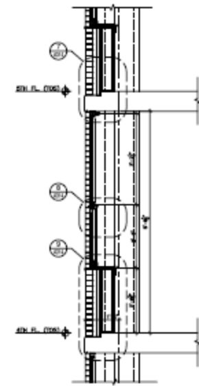
6 PARTIAL WALL SECTION (TYPICAL @ BRICK) SCALE 1/4"=1'-0"
