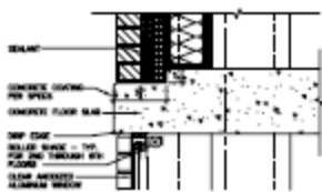
7 WALL SECTION DETAIL (TYPICAL @ BRICK) SCALE 1/4"=1'-0"
