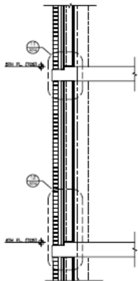
10 PARTIAL WALL SECTION (TYPICAL @ BRICK) SCALE 1/4"=1'-0"
