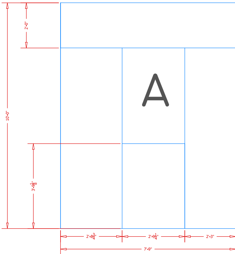
1 Front View 2B Wall G 3/4" = 1' - 0"
