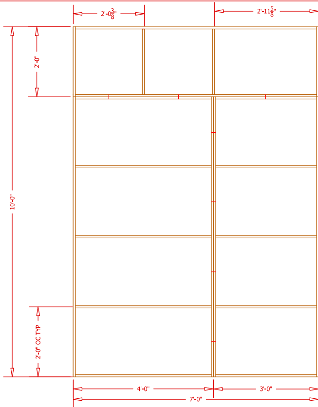
1 Rear View 3A Wall H 3/4" = 1' - 0"
