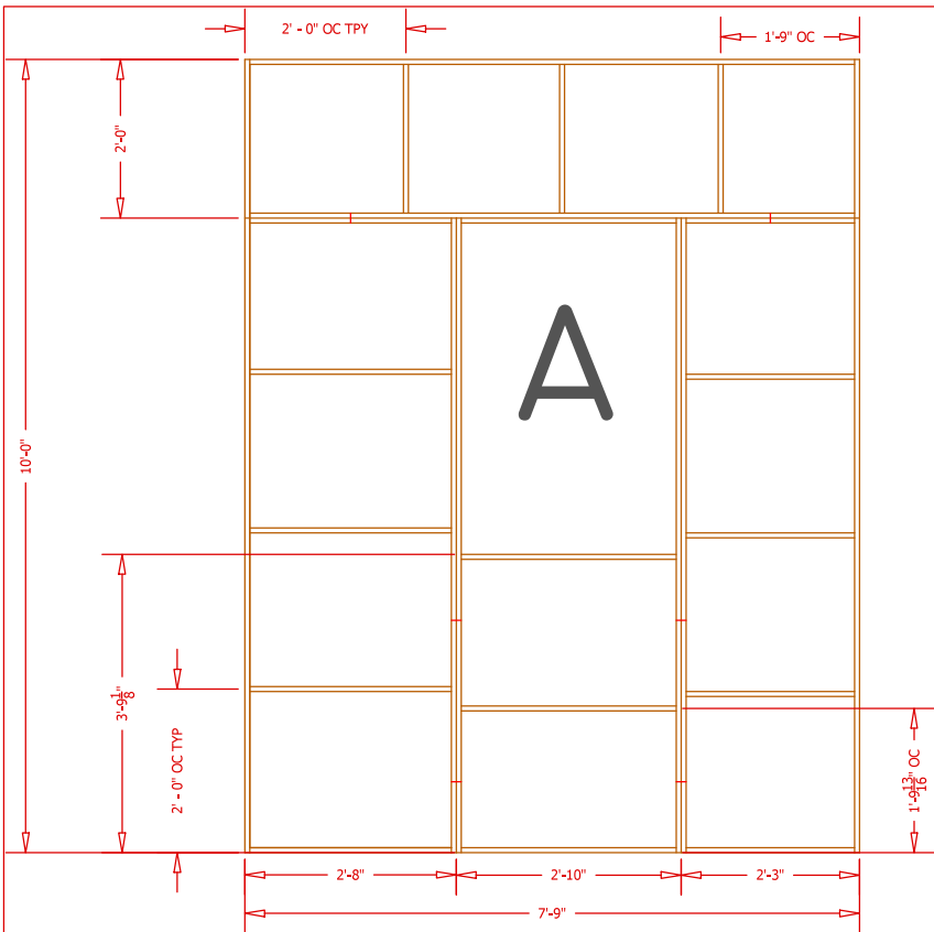
1 Rear View 2A Wall G 3/4" = 1' - 0"
