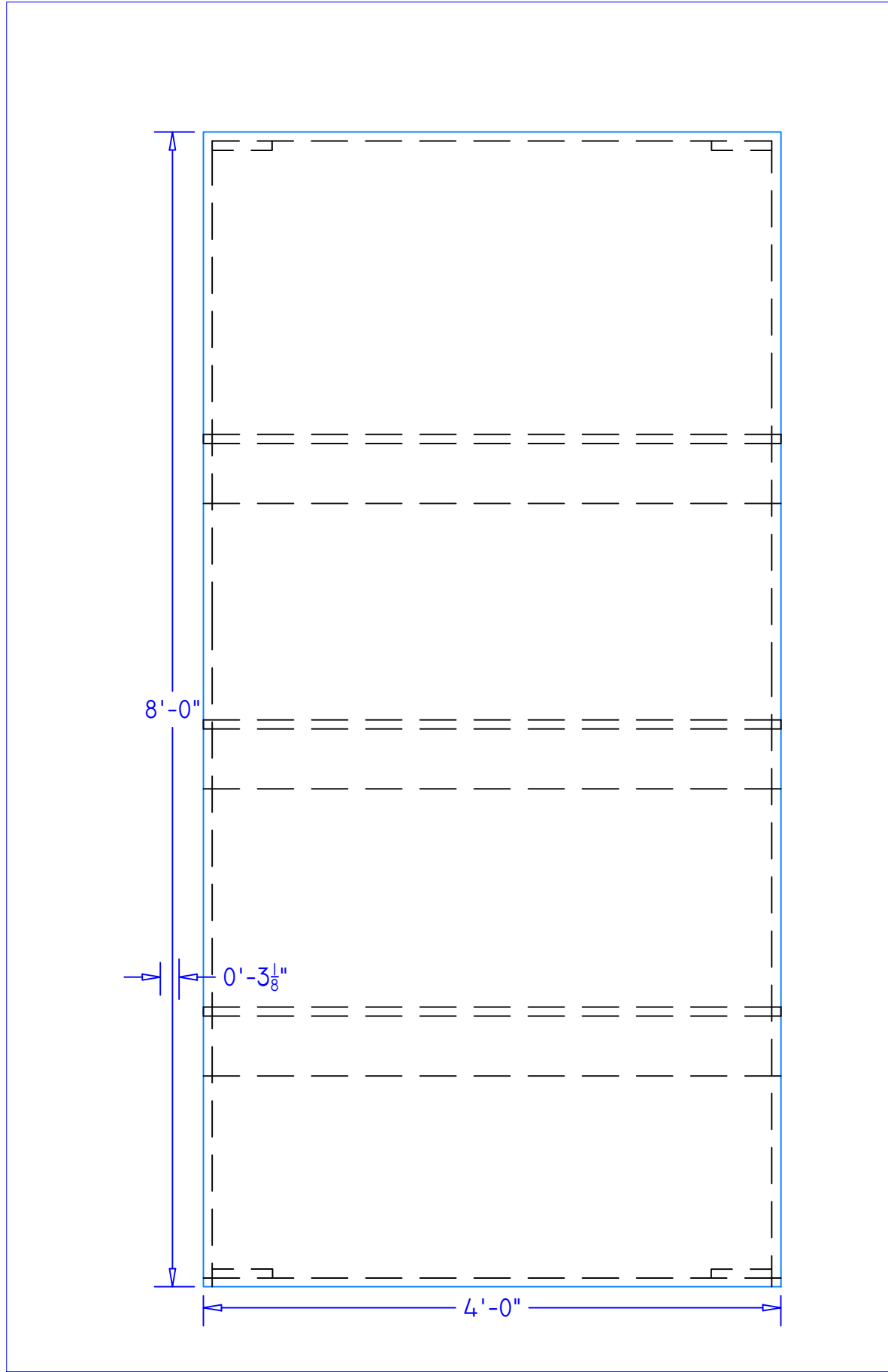
FRONT VIEW
