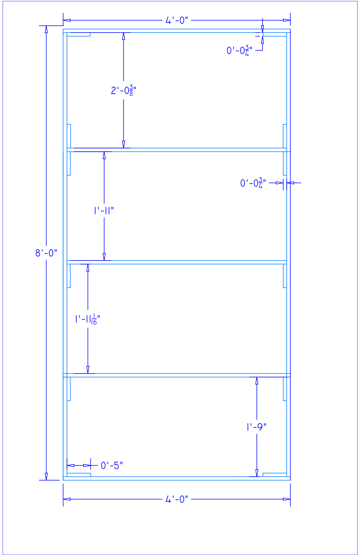
REAR VIEW
