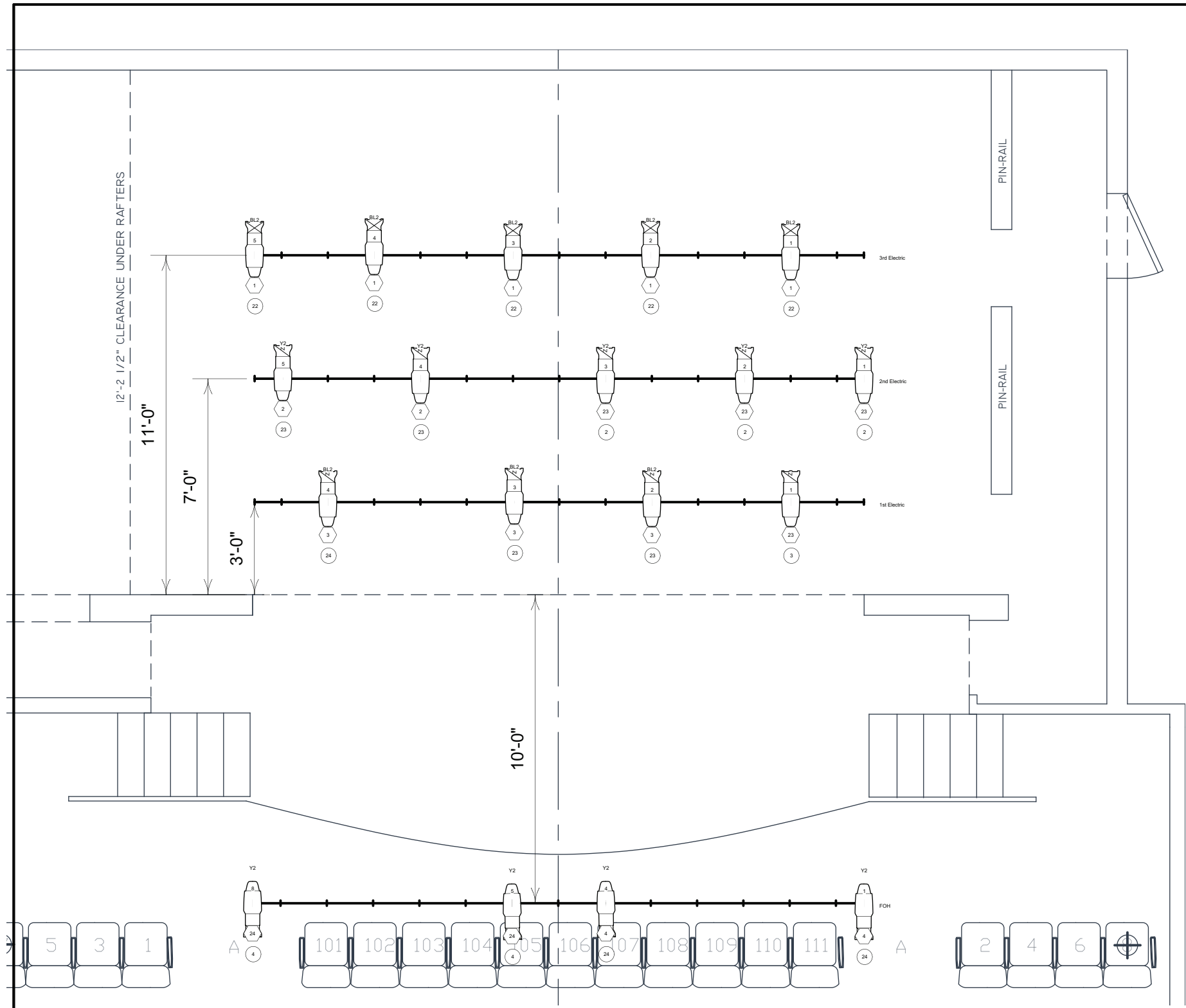
1 LIGHTING PLOT Scale: 1/4" = 1'-0"
