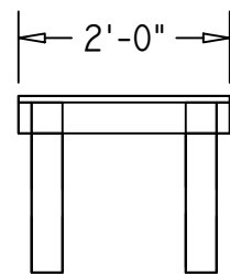
6 Front & Side view(Platform D) 2 Step legs 1/2"-1'
