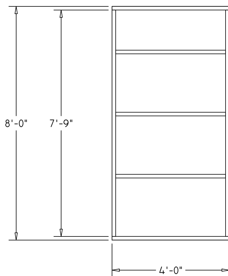
1 Platform construction 1 Platform 1/2"-1'
