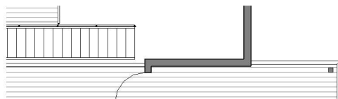
1 BALCONY 1 1/4" = 1'-0"
