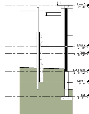
4 BALCONY SECTION 2 1/4" = 1'-0"
