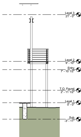
3 BALCONY SECTION 1 1/4" = 1'-0"
