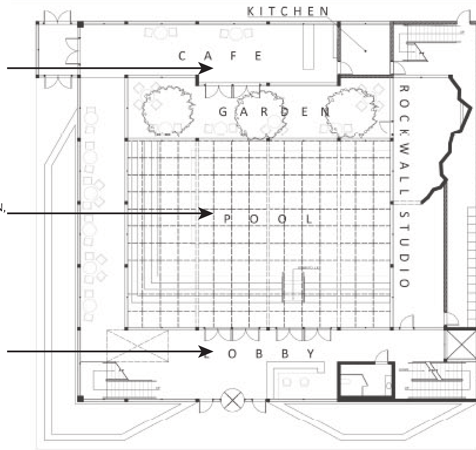
FIRST FLOOR, PROGRAM CONSIST OF CAFE, KITCHEN, POOL, LOBBY, ROCKWALL, AND STUDIO
