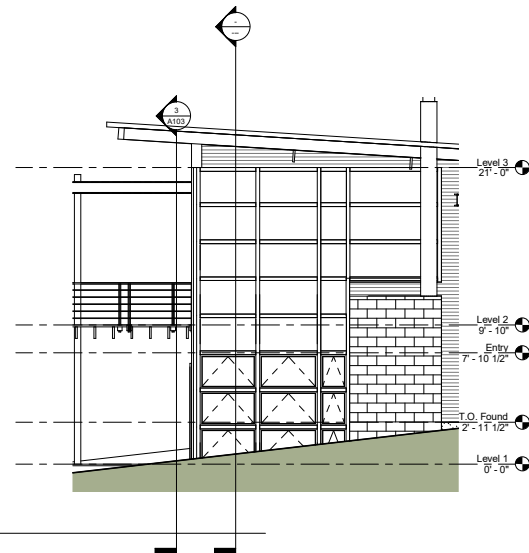
⑥ Callout of North 1/4" = 1'-0"
