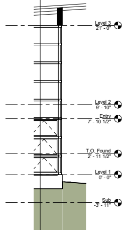
④ CURTAIN WALL SECTION 1/4" = 1'-0"
