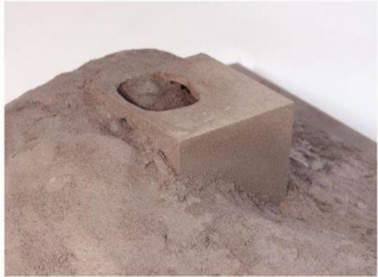
Natural erosion of landscape begins.
