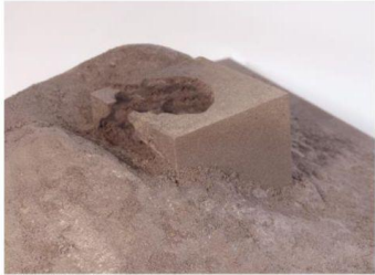
Banking erosion begins.
