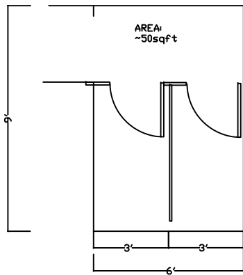
TYP. BATHROOM LAYOUTS SCALE 3/16" = 1'-0"
