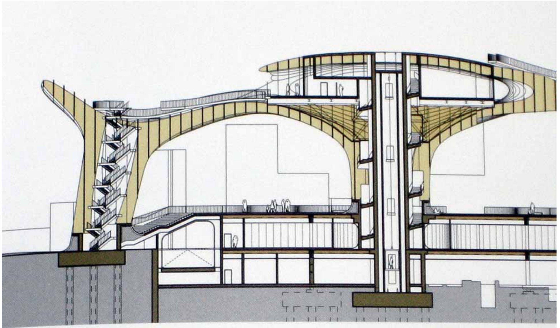
North-south section
