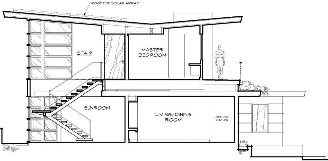
BLDG. SCTN. 0 1 2 4 8 12 16 FEET
