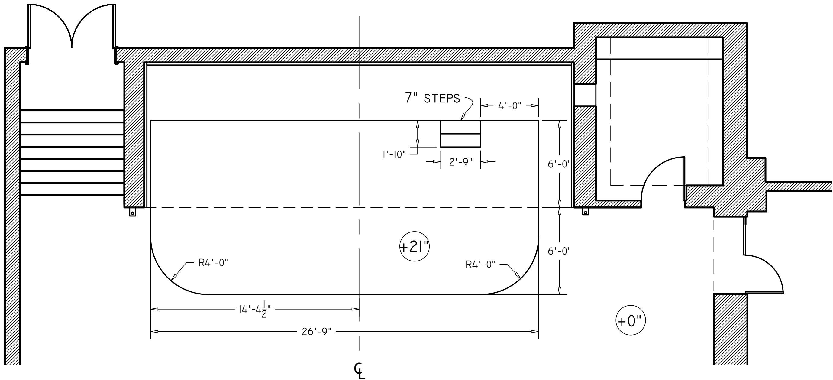
① FINAL PROJECT - GROUND PLAN
