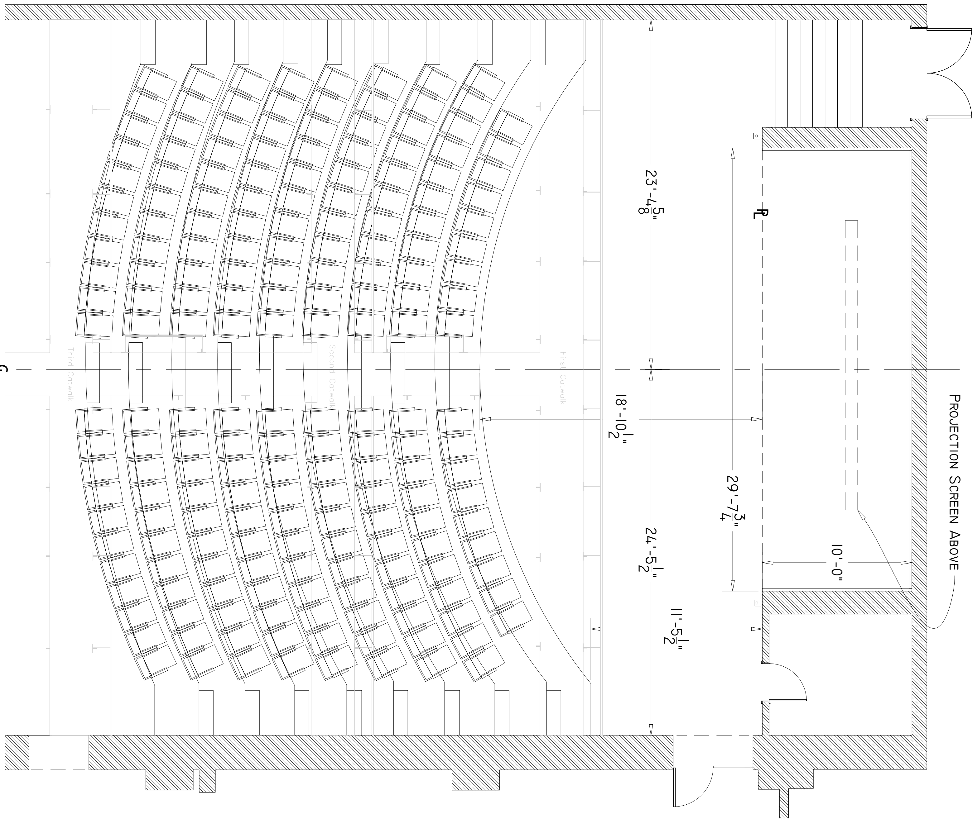
1 GROUND PLAN
