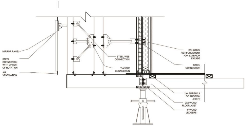
FLOOR DETAIL
