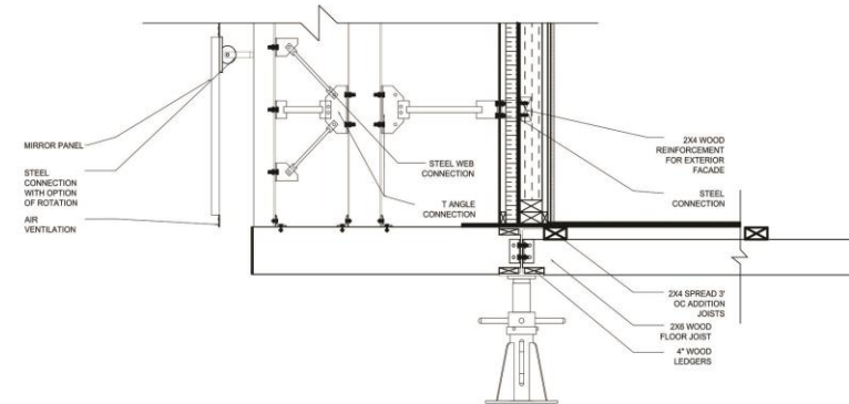
FLOOR DETAIL
