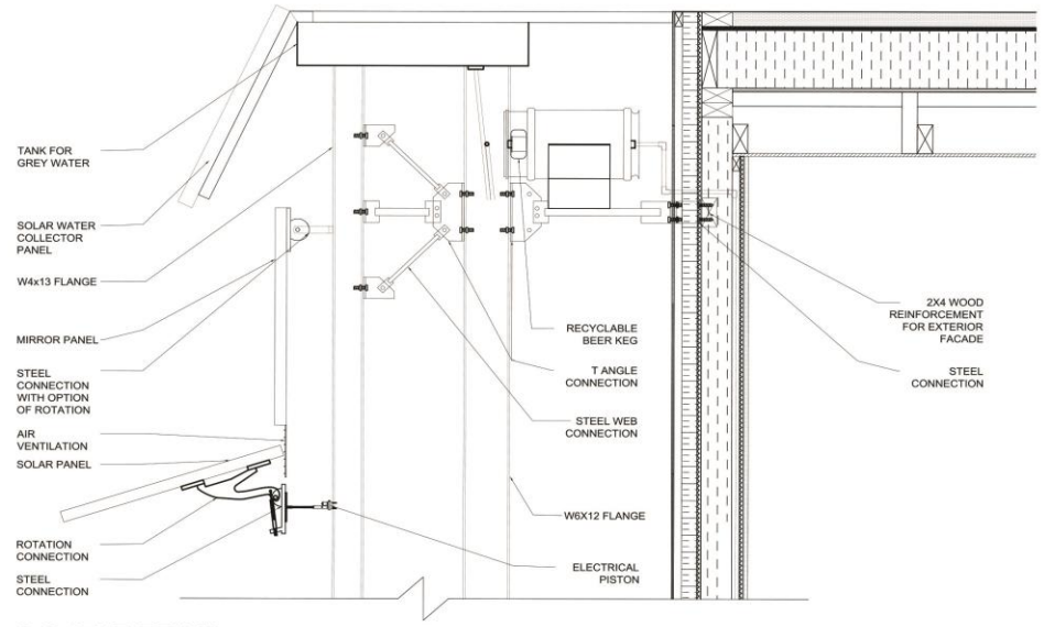
ROOF DETAIL
