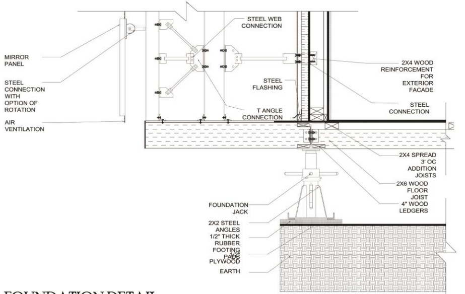
FOUNDATION DETAIL
