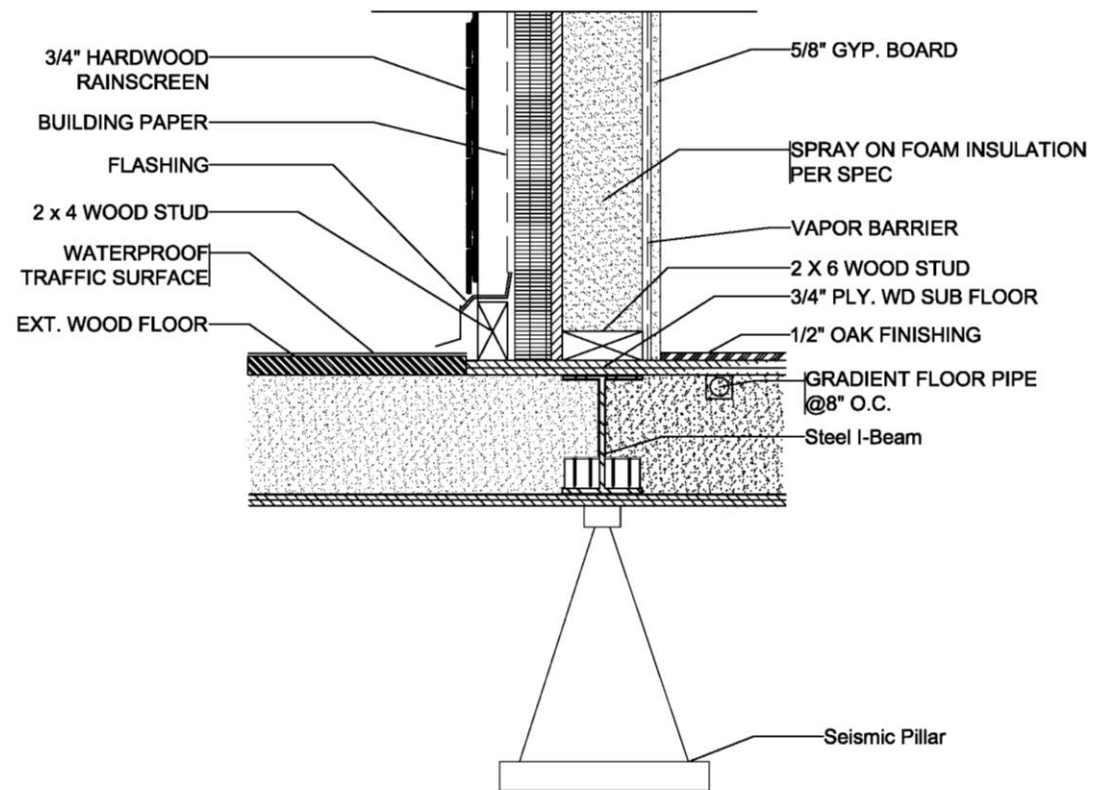
1 WALL TO FLOOR CONNECTION SCALE: 1/4" = 1'-0"
