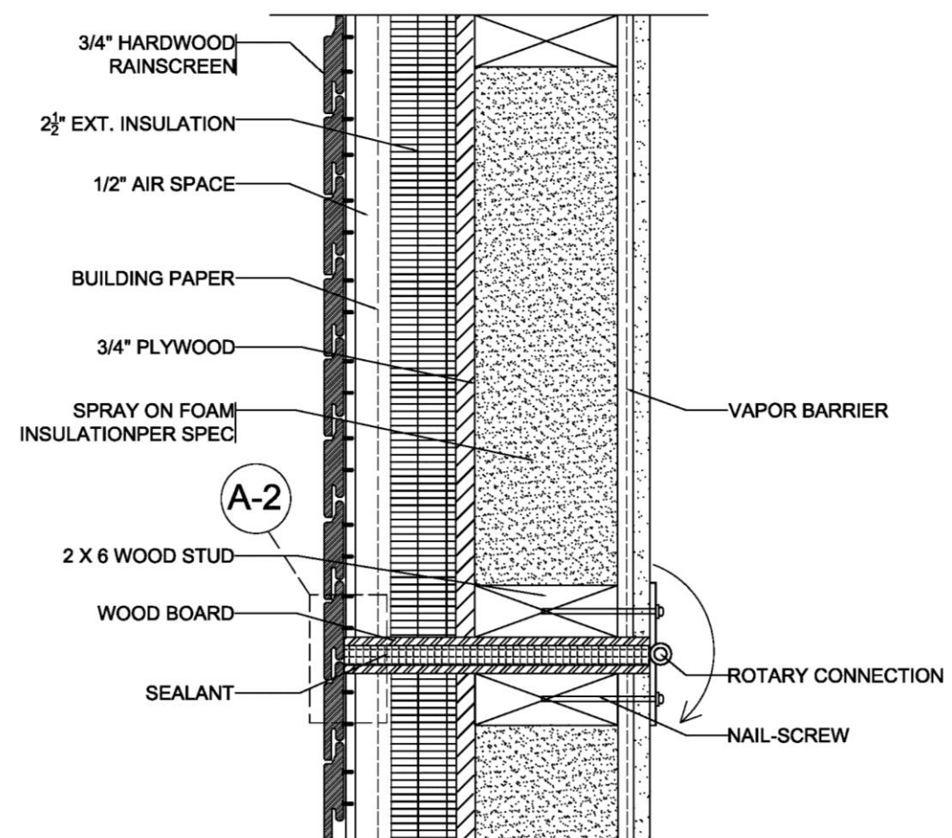
4 FOLDING CONNECTION SCALE: 1/4" = 1'-0"
