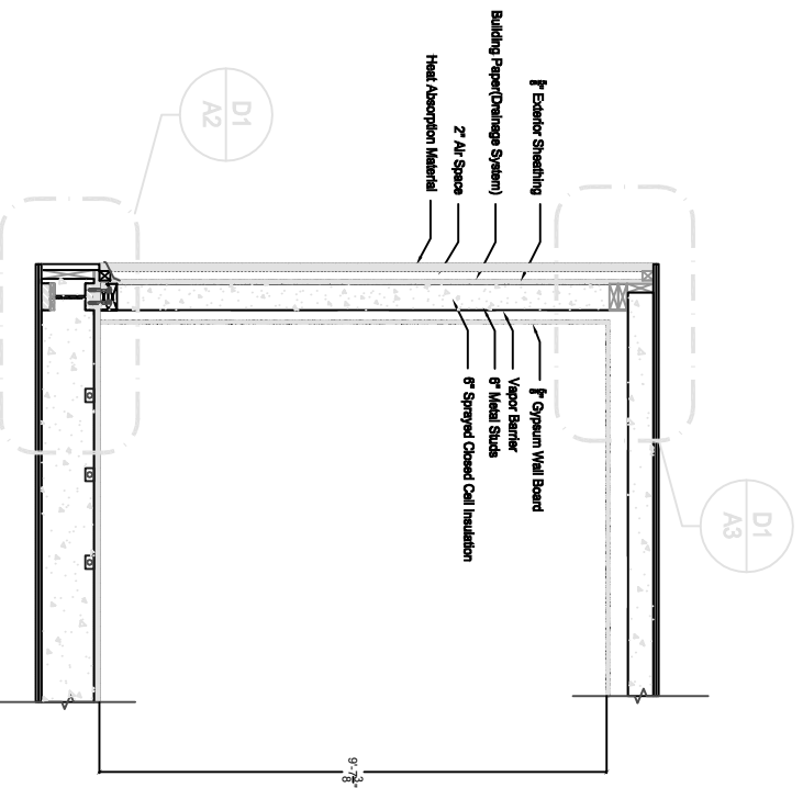
S1 South Wall Section
