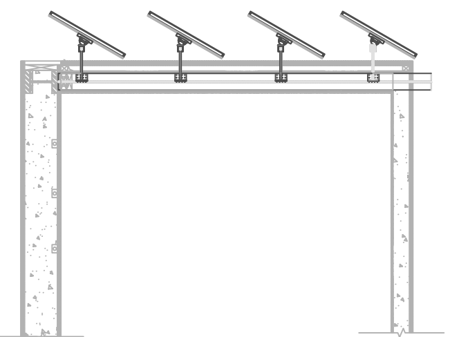
S2 Structural South Section
