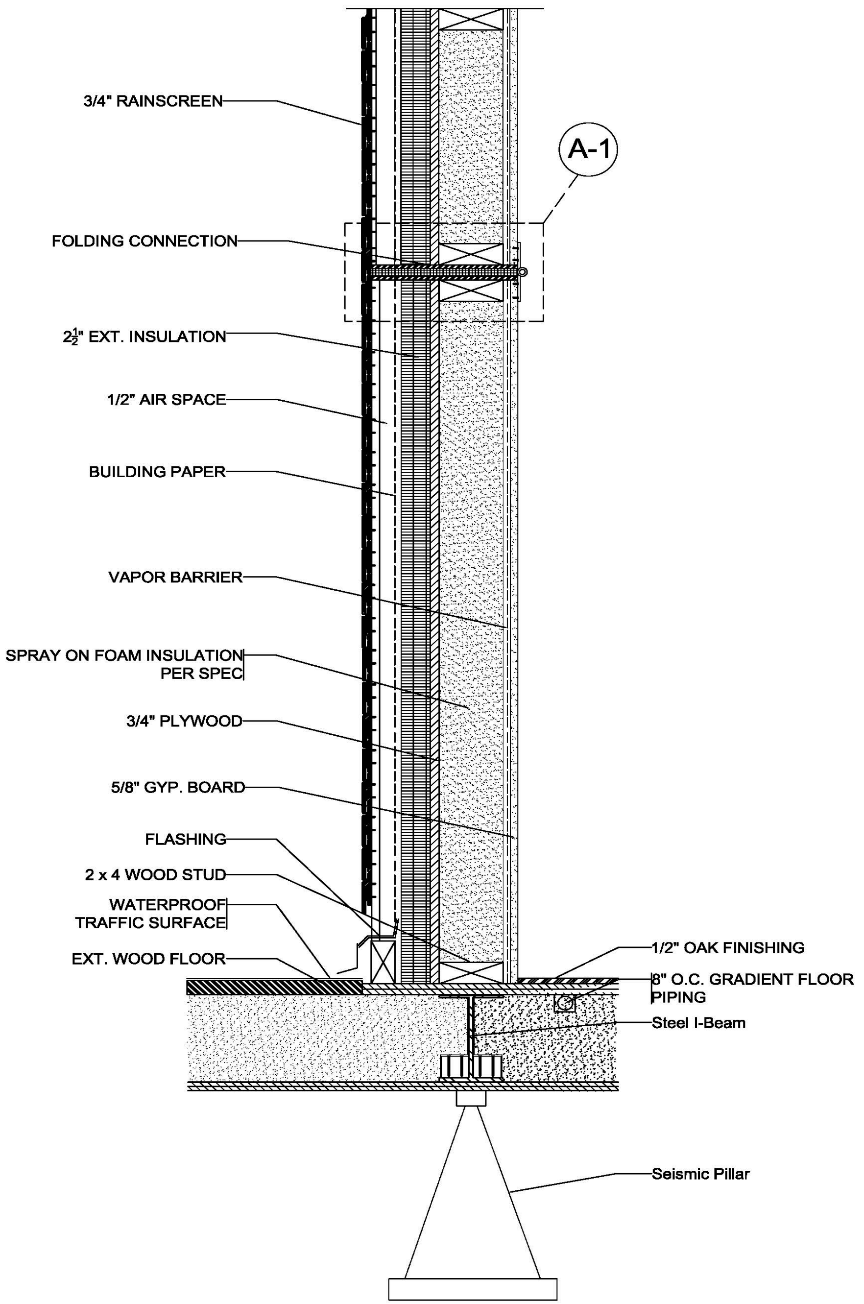
A TYP WALL w/ FOLDING CONNECTION SCALE: 1/4" = 1'-0"
