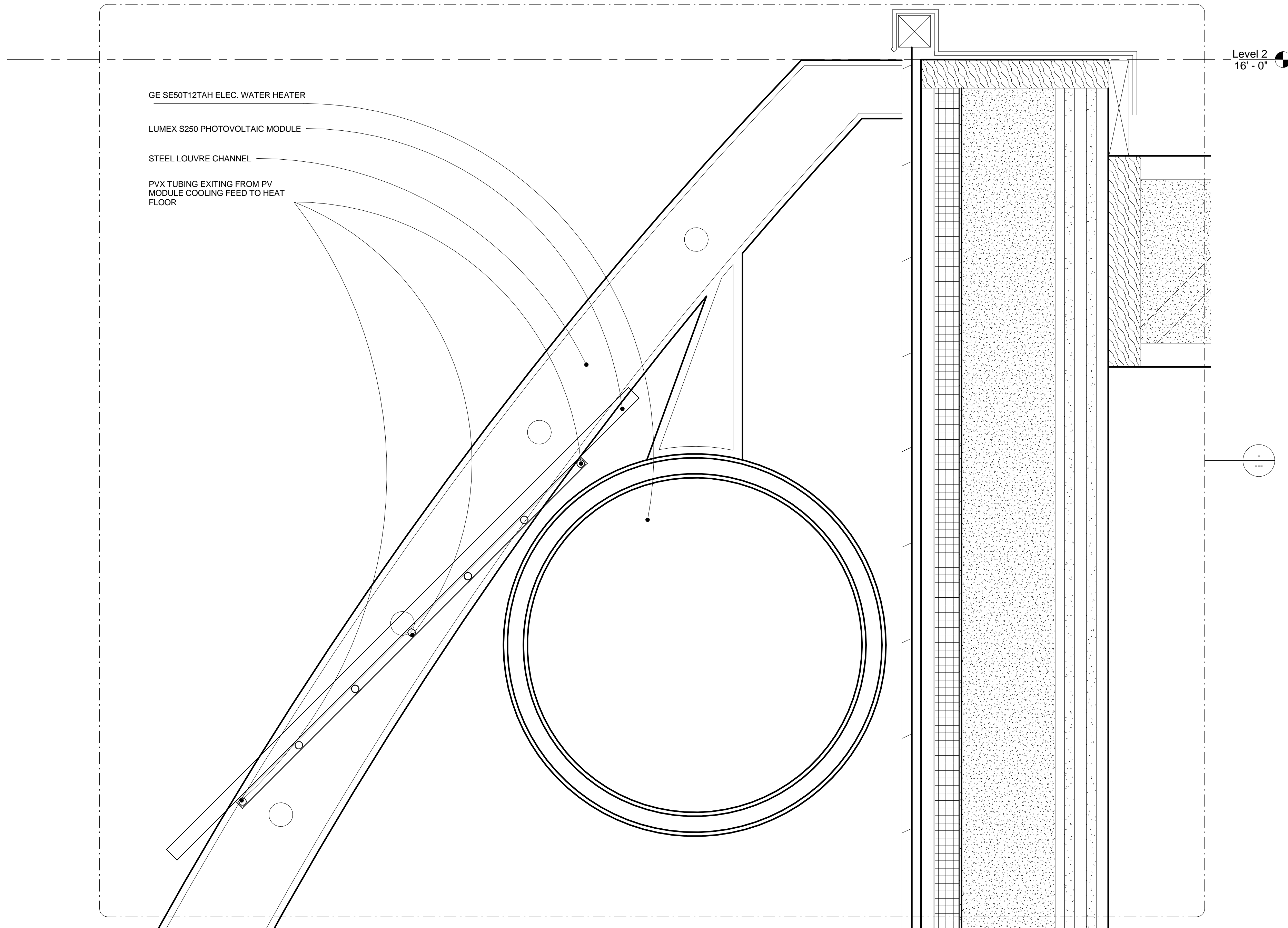
1 Callout A 3" = 1'-0"
