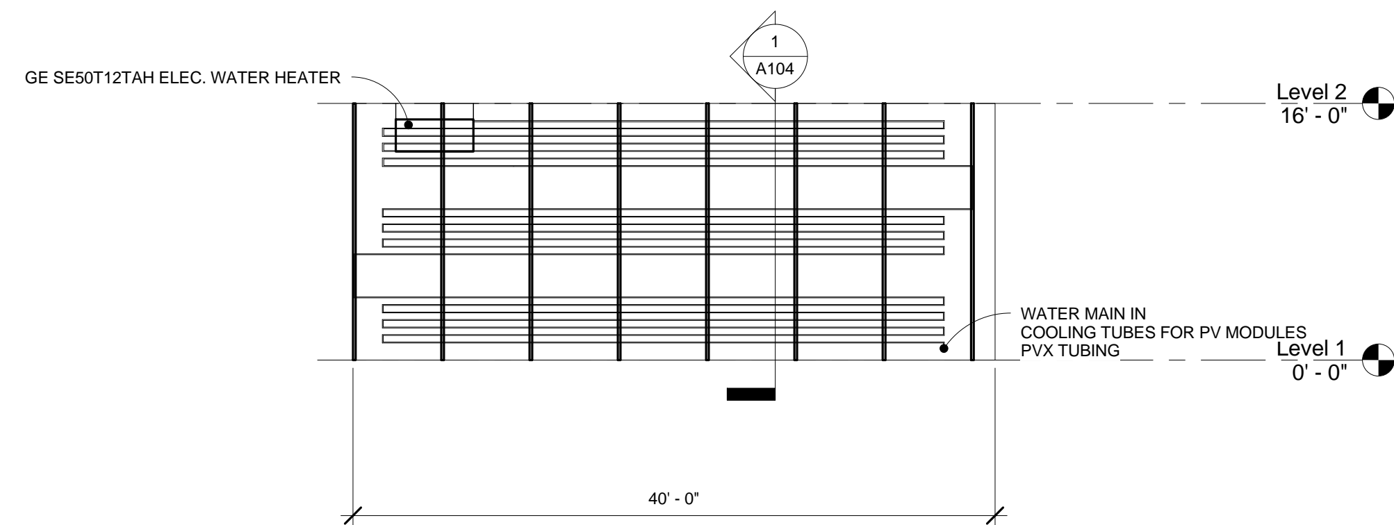
2 PVX Tubing Design 1/8" = 1'-0"
