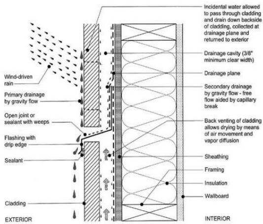
Figure 3 Rainscreen Wall Assembly
