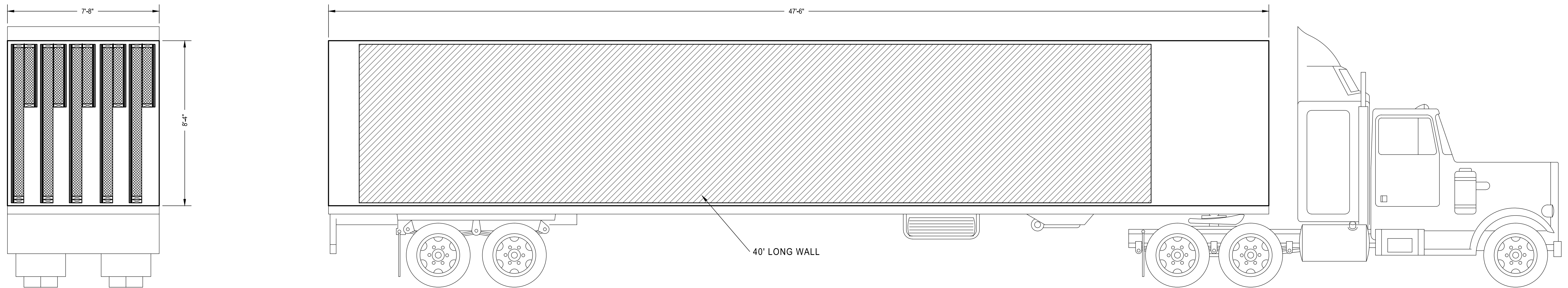
WALLS IN TRAILER 3/8" = 1'-0"
