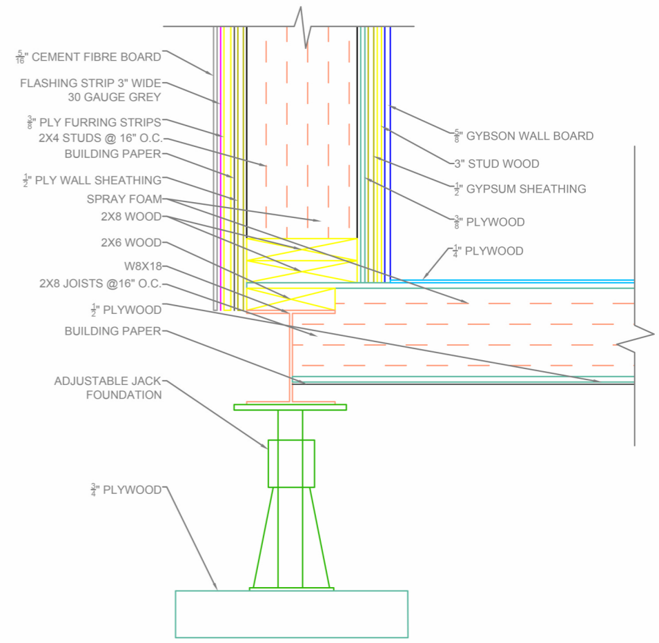
(3) FLOOR SECTION
