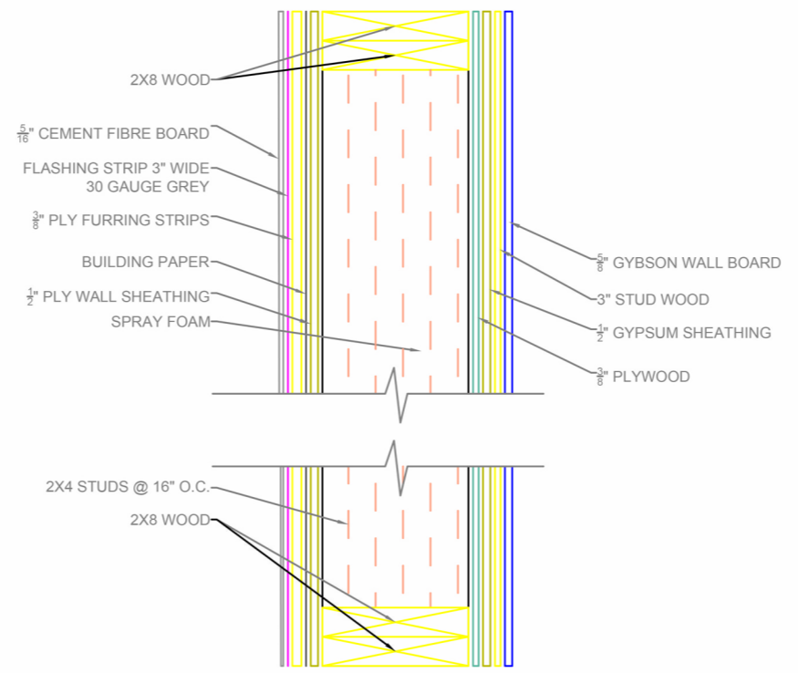
(2) WALL SECTION
