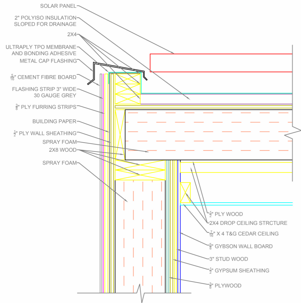
(1) ROOF SECTION
