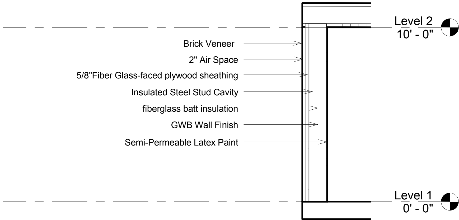
1 Wall Detail 1/4" = 1'-0"
