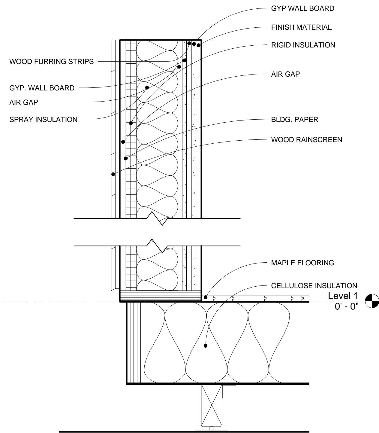
1 Section 1 1 1/2" = 1'-0"
