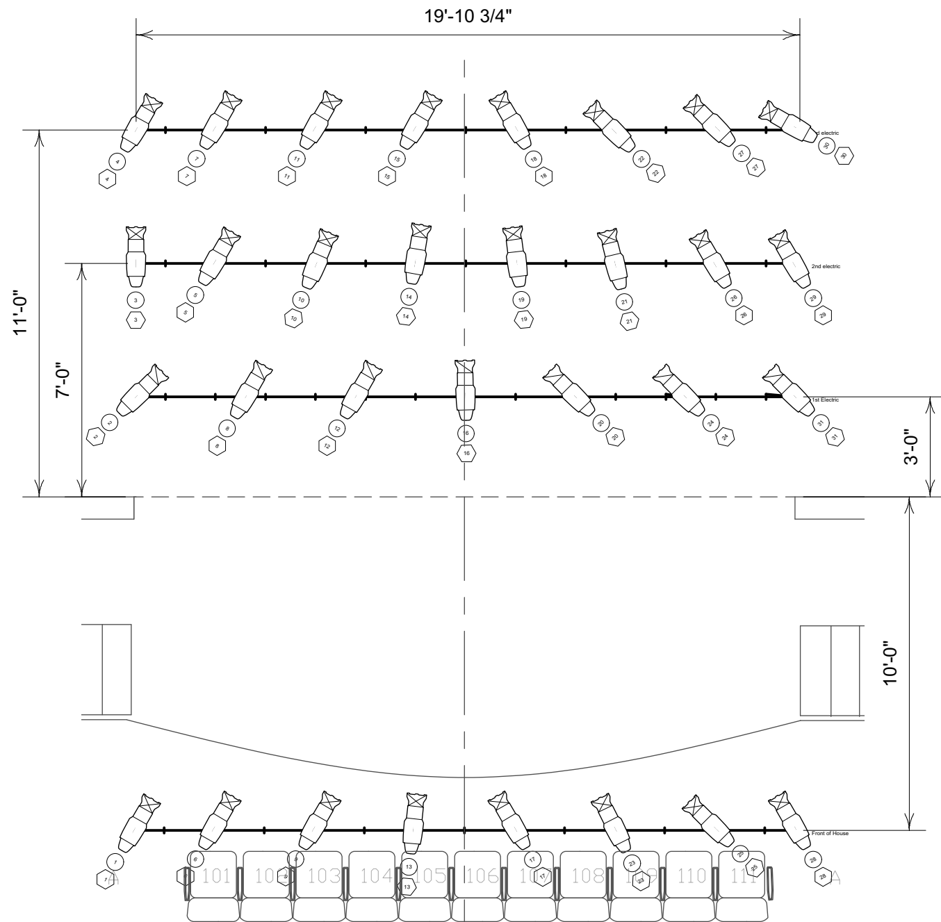
1 Light Plot Scale: 1/4" = 1'-0"
