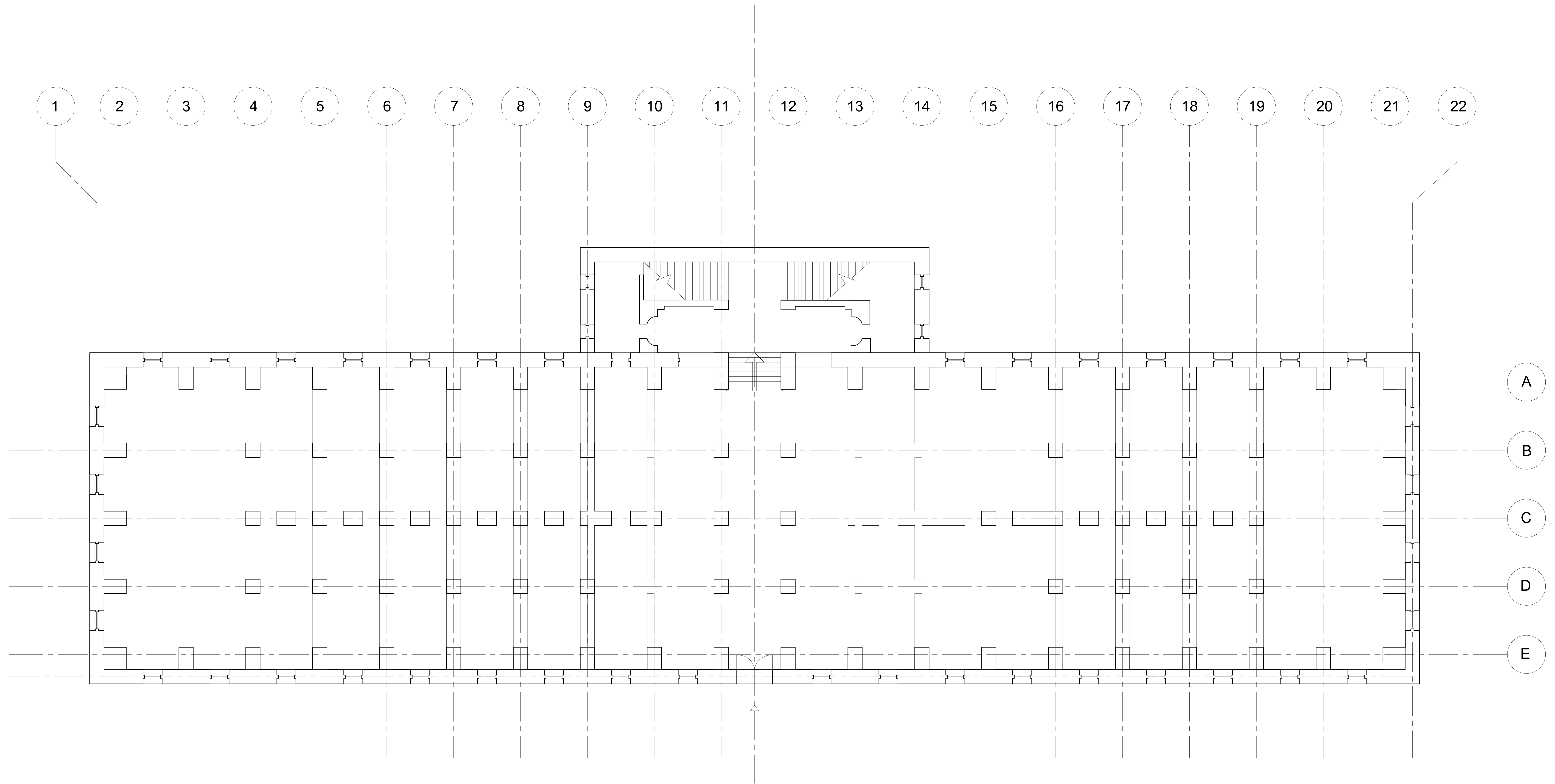
BIBLIOTHEQUE S. GENEVIEVE LOWER FLOOR PLAN Arch1230_MONTGOMERY_2017_OCT.10 PARMAR, POOJA
