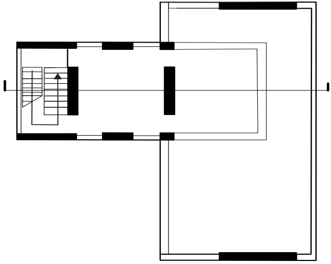
Top Floor Plan
