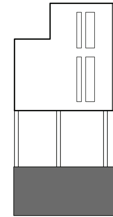
East Elevation
